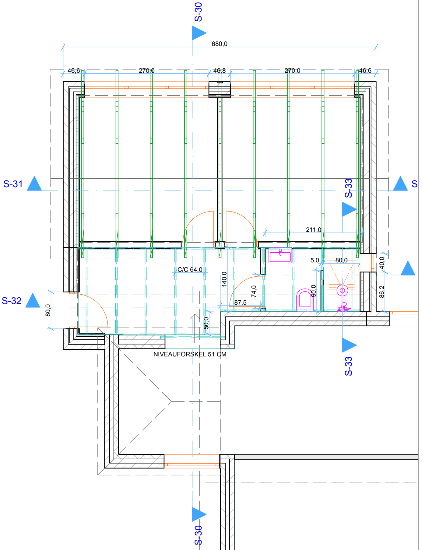
0. Ground Floor 1:50
